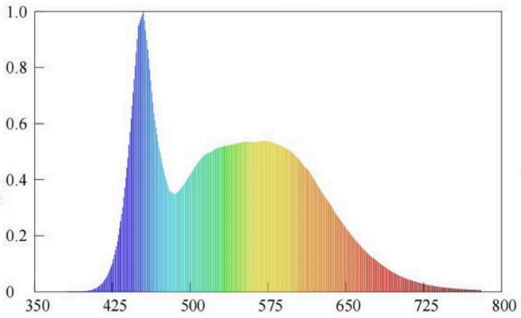
Spectral power distribution(6500k)
